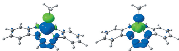
Figure 5. Spin density (IsoValue=0.01) of triplet (left) and singlet (right) [(dadi)Cr=NMe]. Note for the triplet the positive spin density on the metal ( \rho_{\text{spin}} \approx +2e^- ) and dadi ligand ( \rho_{\text{spin}} \approx +1e^- ), and the negative spin density on the imidyl nitrogen ( \rho_{\text{spin}} \approx -1e^- ). For the broken-symmetry singlet, the spin density on the imidyl ( \rho_{\text{spin}} \approx +1e^- ) and dadi ( \rho_{\text{spin}} \approx +1e^- ) ligand are positive, while the Cr has negative spin density ( \rho_{\text{spin}} \approx -2e^- ).
